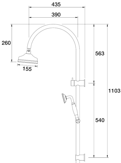
Tudor Wall Shower Divertor on Rail Gooseneck Top Connection Porcelain Handle C31.063.5.23 - Gunmetal
