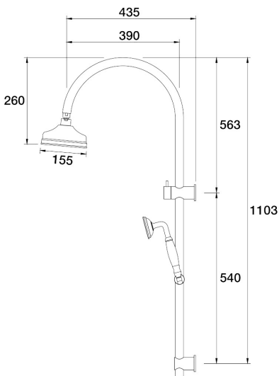
Tudor Wall Shower Divertor on Rail Gooseneck Top Connection Porcelain Handle C31.063.5.41 - Brushed Brass
