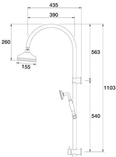
Tudor Wall Shower Divertor on Rail Gooseneck Bottom Connection Porcelain Handle C31.063.6.01 - Chrome
