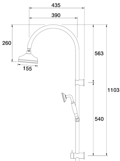
Tudor Wall Shower Divertor on Rail Gooseneck Bottom Connection Porcelain Handle C31.063.6.11 - 23k Gold
