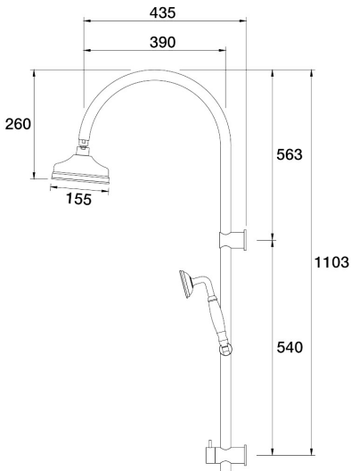
Tudor Wall Shower Divertor on Rail Gooseneck Bottom Connection Porcelain Handle C31.063.6.54 - Volcanic Grey
