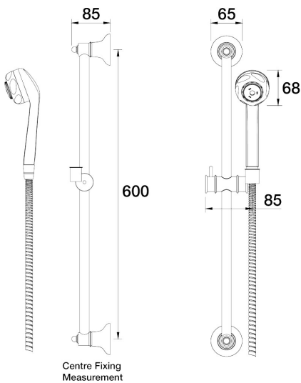
Bell Handshower on Rail Three Function C32.052.1.01 - Chrome
