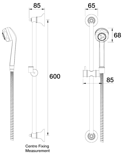
Bell Handshower on Rail Three Function C32.052.1.07 - Chrome / Victorian Green
