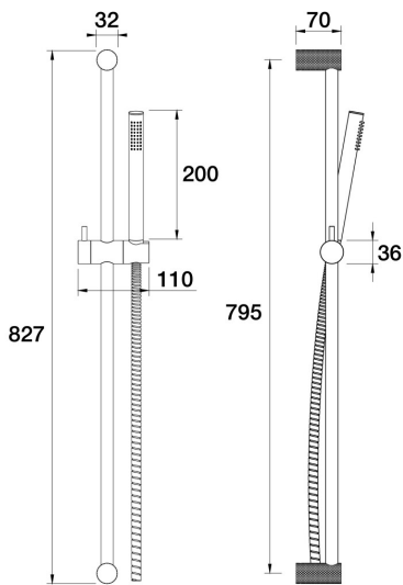
IDK Handshower on Rail C38.052.1.32 - Midnight Black
