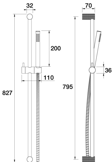
Opus Handshower on Rail C45.052.1.42 - Brushed Copper
