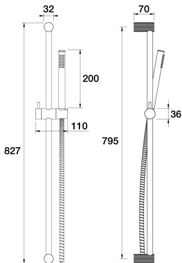
Opus Handshower on Rail C45.052.1.43 - Brass
