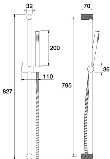
Opus Handshower on Rail C45.052.1.67 - Vintage Brass
