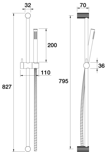
Opus Handshower on Rail Lane C45.052.2.32 - Midnight Black
