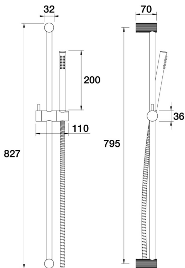
Opus Handshower on Rail Lane C45.052.2.41 - Brushed Brass
