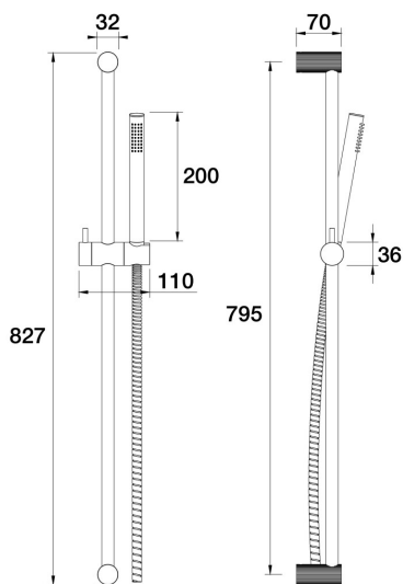
Opus Handshower on Rail Lane C45.052.2.42 - Brushed Copper
