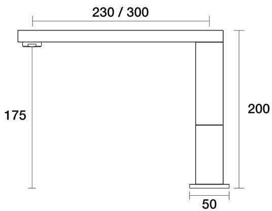
Burj Spa Hob Swivel Outlet D20.042.1.02 - Brushed Chrome
