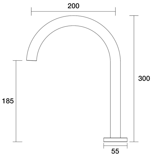
Lugano Sink Hob Swivel Outlet D22.032.1.54 - Volcanic Grey
