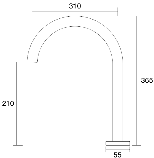
Lugano Sink Hob Swivel Outlet X/Large D22.032.2.01 - Chrome
