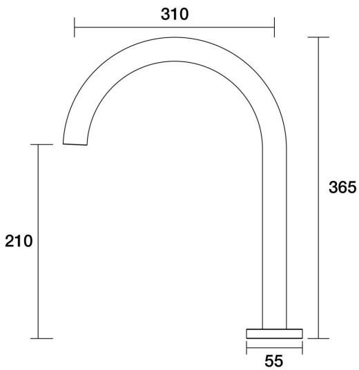
Lugano Sink Hob Swivel Outlet X/Large D22.032.2.01 - Chrome
