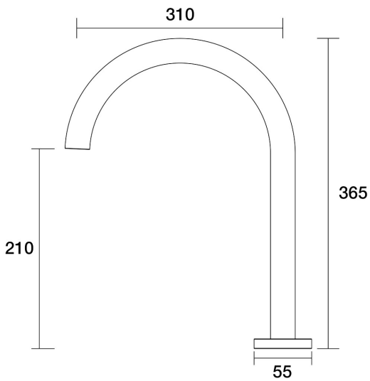
Lugano Sink Hob Swivel Outlet X/Large D22.032.2.42 - Brushed Copper
