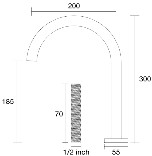
Lugano Sink Hob Swivel Outlet For Basin D22.032.3.01 - Chrome
