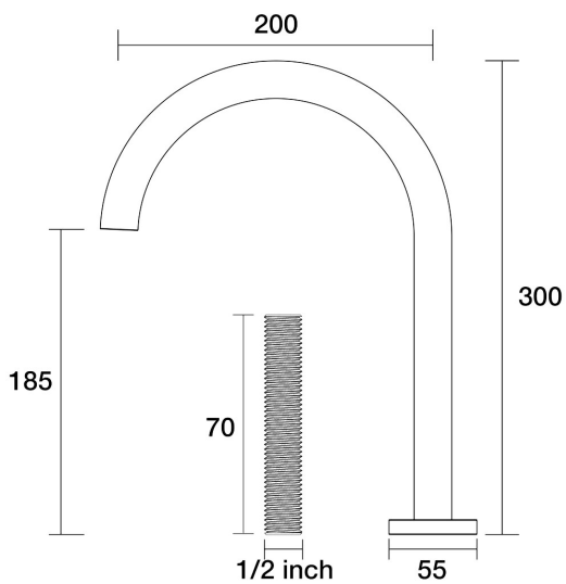
Lugano Sink Hob Swivel Outlet For Basin D22.032.3.41 - Brushed Brass
