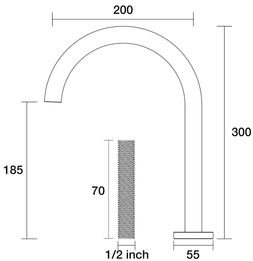
Lugano Sink Hob Swivel Outlet For Basin D22.032.3.45 - Native Brass
