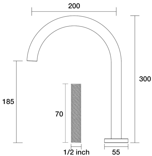
Lugano Sink Hob Swivel Outlet For Basin D22.032.3.47 - Luminick
