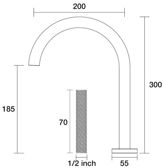
Lugano Sink Hob Swivel Outlet For Basin D22.032.3.75 - Forest Mist
