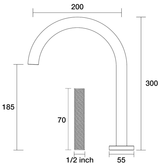
Lugano Sink Hob Swivel Outlet For Basin D22.032.3.77 - Oud Bronze
