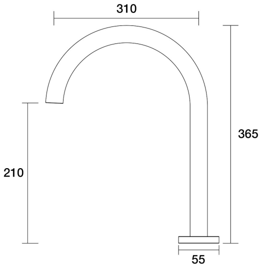
Lugano Spa Hob Swivel Outlet X/Large D22.042.2.68 - Autumn Bronze
