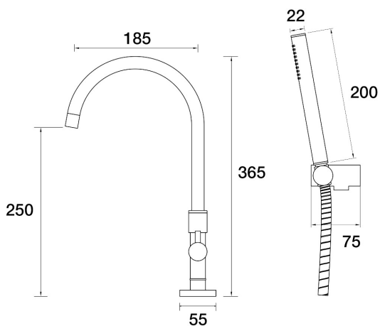
Lugano Spa Hob Swivel Outlet Divertor Gooseneck Outlet with Handshower D22.042.3.75 - Forest Mist
