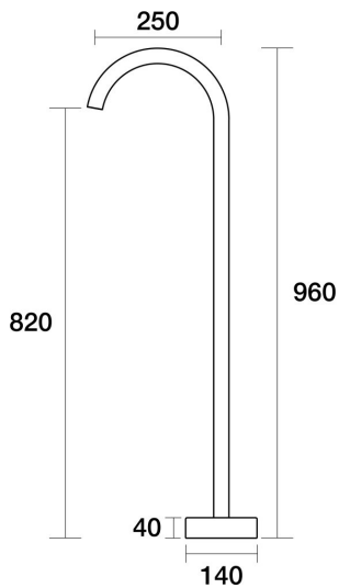
Lugano Floor Filler Fixed Outlet 250mm D22.051.1.01 - Chrome
