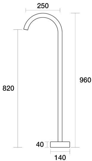
Lugano Floor Filler Fixed Outlet 250mm D22.051.1.43 - Brass
