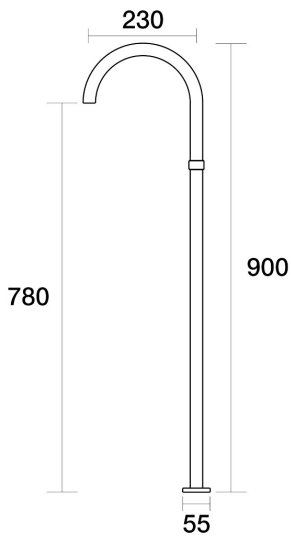
Lugano Floor Filler Swivel Outlet 230mm D22.052.1.54 - Volcanic Grey
