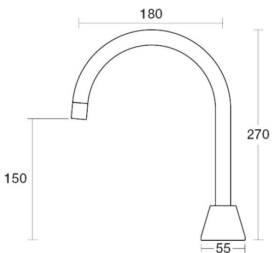
Forme Sink Hob Swivel Outlet D27.032.1.02 - Brushed Chrome
