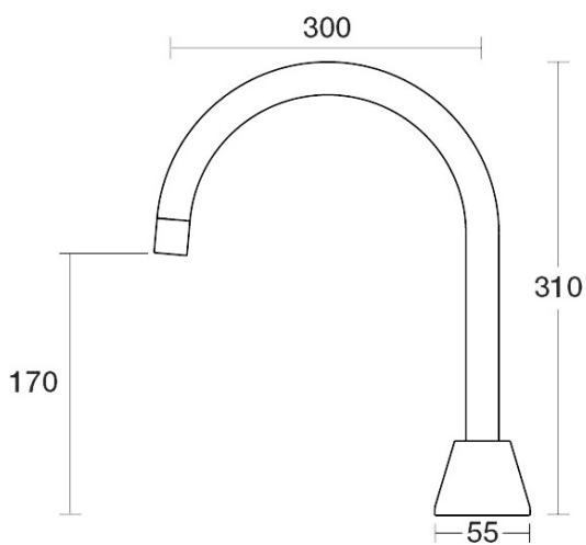
Forme Sink Hob Swivel Outlet X/Large D27.032.2.02 - Brushed Chrome
