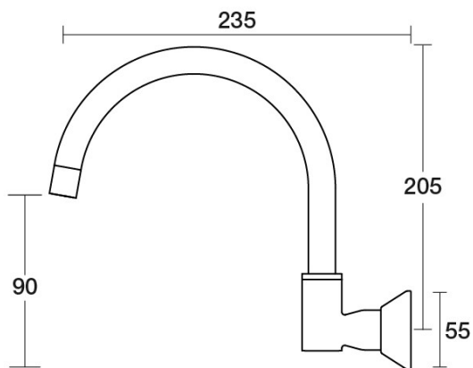
Forme Sink Wall Swivel Outlet D27.034.1.24 - Brushed Gunmetal
