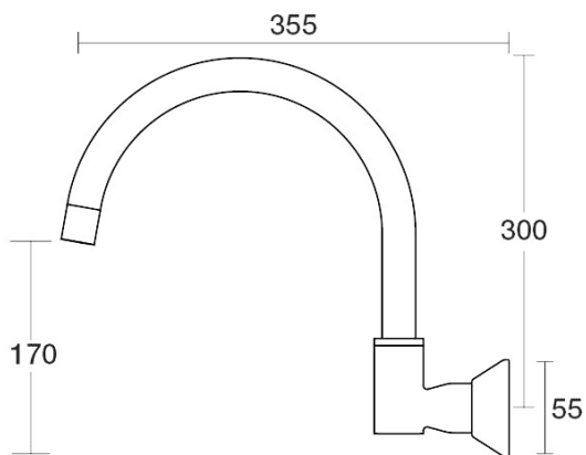
Forme Sink Wall Swivel Outlet X/Large D27.034.2.01 - Chrome
