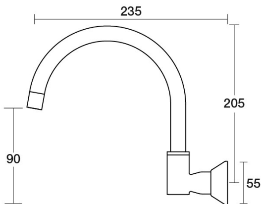
Forme Spa Wall Swivel Outlet D27.044.1.25 - Brushed Nickel
