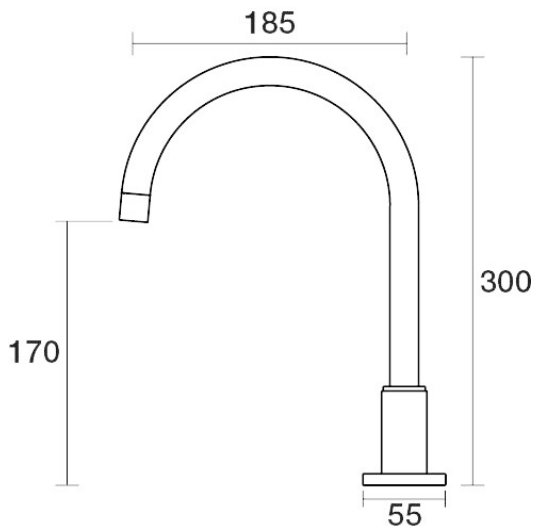
Portsea Sink Hob Swivel Outlet D29.032.1.01 - Chrome
