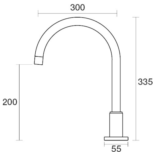
Portsea Sink Hob Swivel Outlet X/Large D29.032.2.02 - Brushed Chrome
