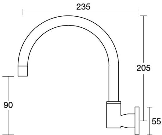
Portsea Sink Wall Swivel Outlet D29.034.1.23 - Gunmetal
