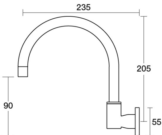
Portsea Sink Wall Swivel Outlet D29.034.1.43 - Brass
