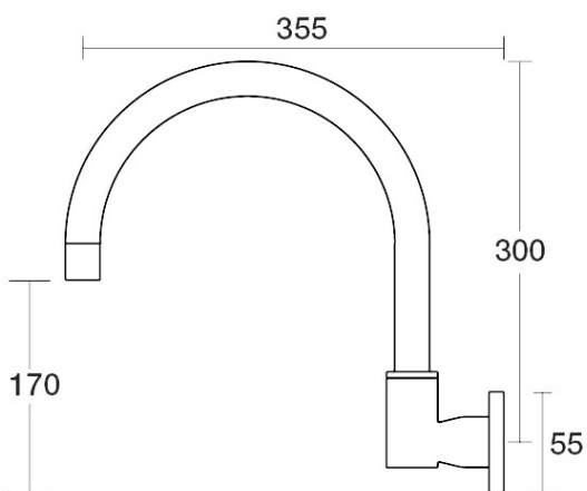
Portsea Sink Wall Swivel Outlet X/Large D29.034.2.23 - Gunmetal
