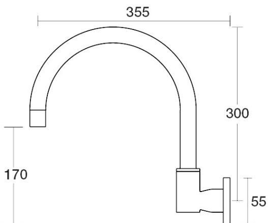
Portsea Sink Wall Swivel Outlet X/Large D29.034.2.52 - Burnished
