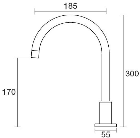
Portsea Spa Hob Swivel Outlet D29.042.1.23 - Gunmetal
