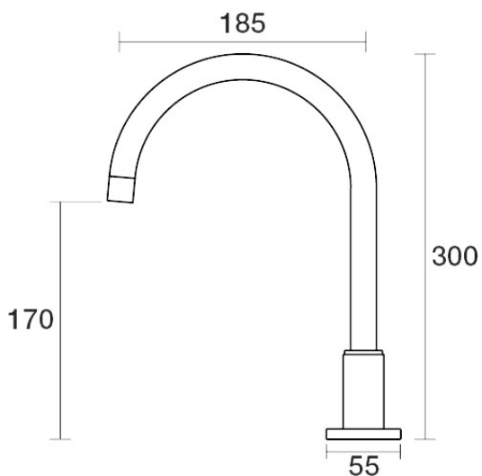
Portsea Spa Hob Swivel Outlet D29.042.1.45 - Native Brass
