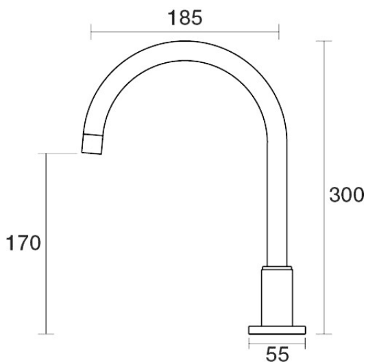
Portsea Spa Hob Swivel Outlet D29.042.1.57 - Matt Nickel
