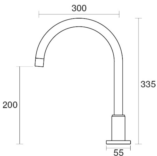
Portsea Spa Hob Swivel Outlet X/Large D29.042.2.67 - Vintage Brass
