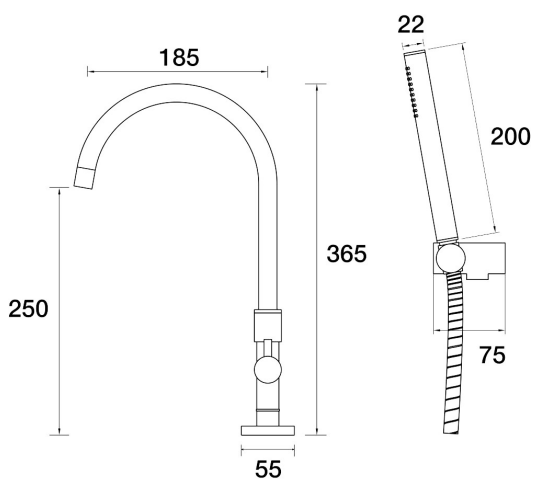
Portsea Spa Hob Swivel Outlet Divertor Outlet with Handshower & Bracket D29.042.3.11 - 23k Gold
