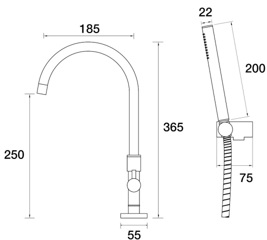
Portsea Spa Hob Swivel Outlet Divertor Outlet with Handshower & Bracket D29.042.3.68 - Autumn Bronze
