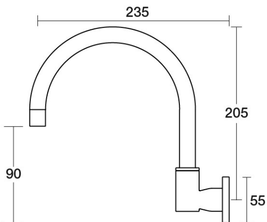
Portsea Spa Wall Swivel Outlet D29.044.1.11 - 23k Gold
