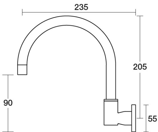
Portsea Spa Wall Swivel Outlet D29.044.1.45 - Native Brass
