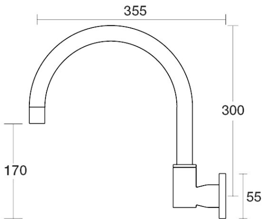
Portsea Spa Wall Swivel Outlet X/Large D29.044.2.67 - Vintage Brass
